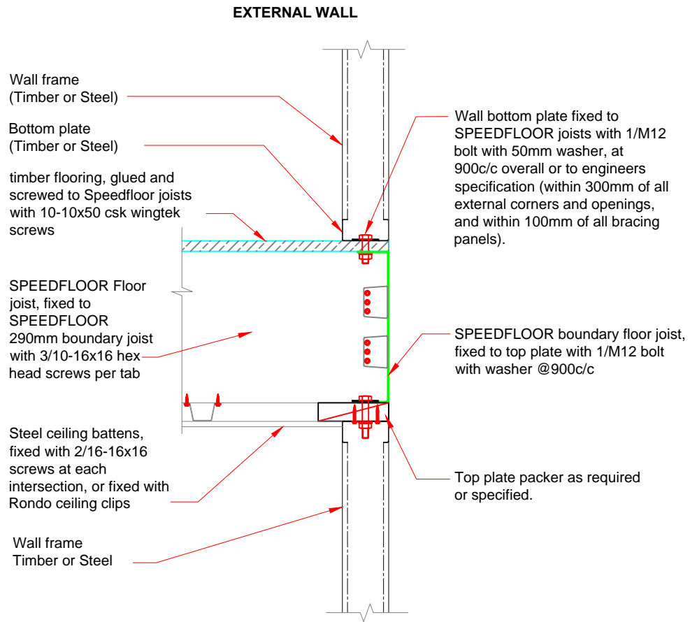
MFD 1A - 290 SPEEDFLOOR joist to steel wall
